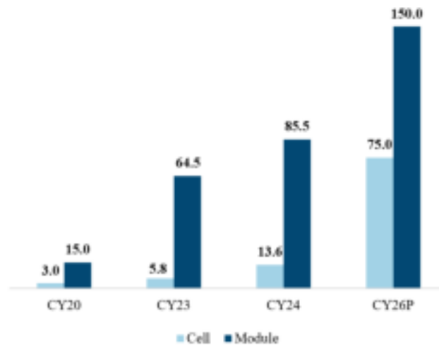
Solar cell and module manufacturing capacity in India (GW, CY20-26P)
